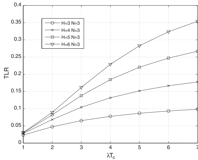
Fig. 9. TLR results for FSA with 8 slots and Poisson arrivals, N=3 and H=3 to H=6 .
