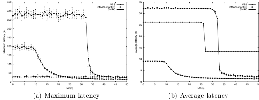
Fig. 5. Single-hop configuration (average \pm 99% confidence interval)
