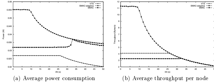
Fig. 6. Power consumption and throughput for single hop (average \pm 99% confidence interval)
